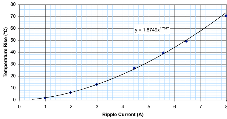
THQ1025183 Temp Rise (free air) vs. 200 Hz Ripple Current
