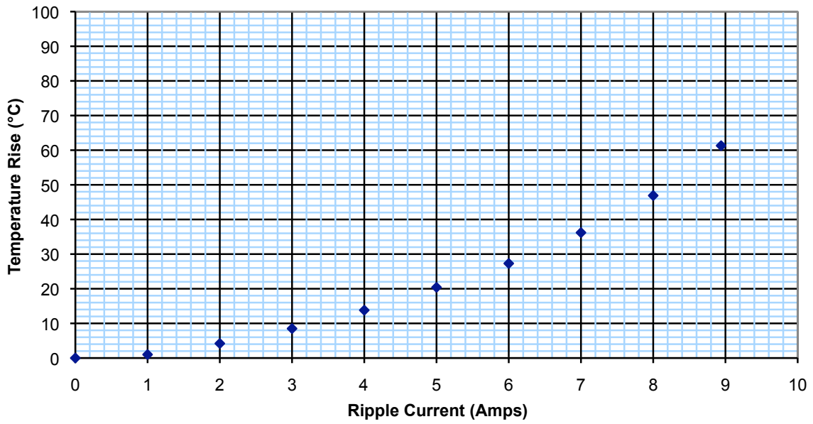
THQ4 Temp Rise (free air) vs. 200Hz Ripple Current
