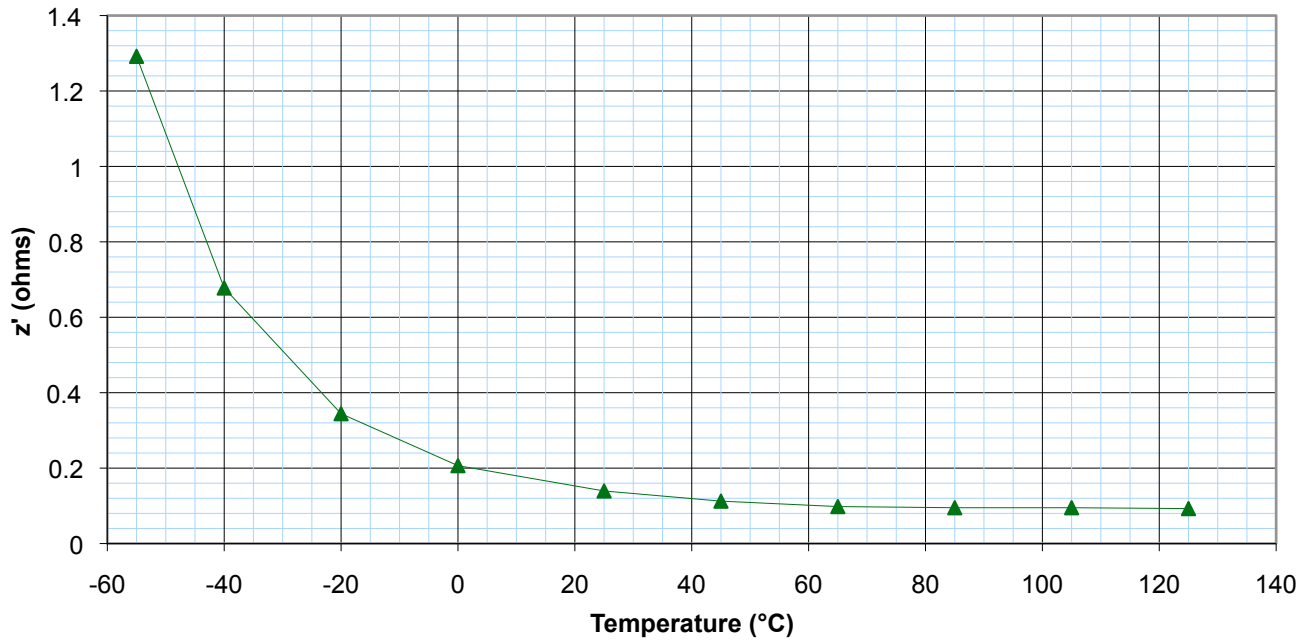
THQA2060871 (1kHz)
